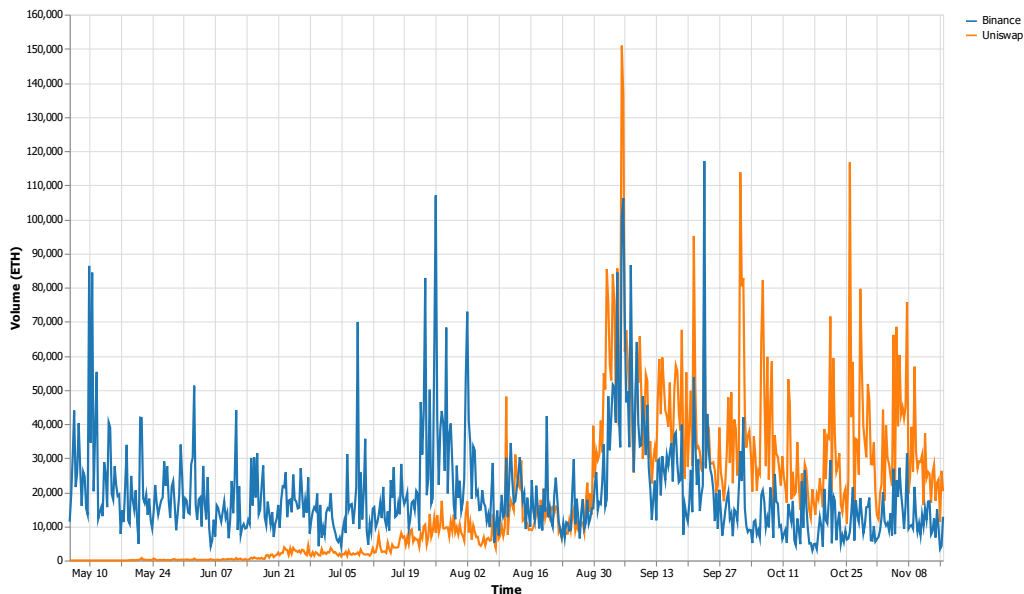
Figure 11. Trading volume of USDC/ETH on Uniswap (orange) and Binance (blue). The graph shows the trading volume excluding flash loans in ETH. Trading volume is aggregated over rolling eight hour intervals.
