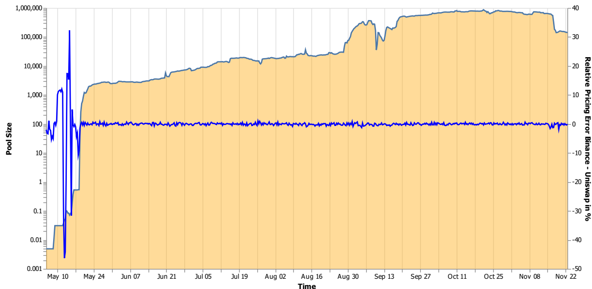
Figure 9. Pricing error and pool size Pricing difference for the USDC/ETH pair when comparing Binance to Uniswap in percent of the Binance price (blue line, right axis) and pool size of the Uniswap USDC/ETH pool (orange, log-scale, left axis).
