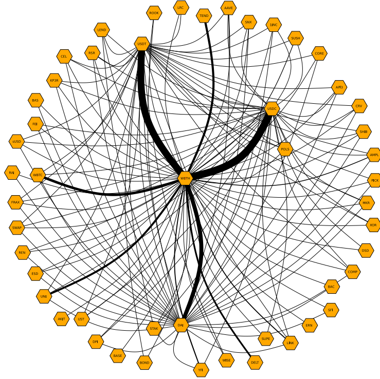
Figure 5. Network graph of pools between all tokens that are part of the 50 largest pools by volume.
