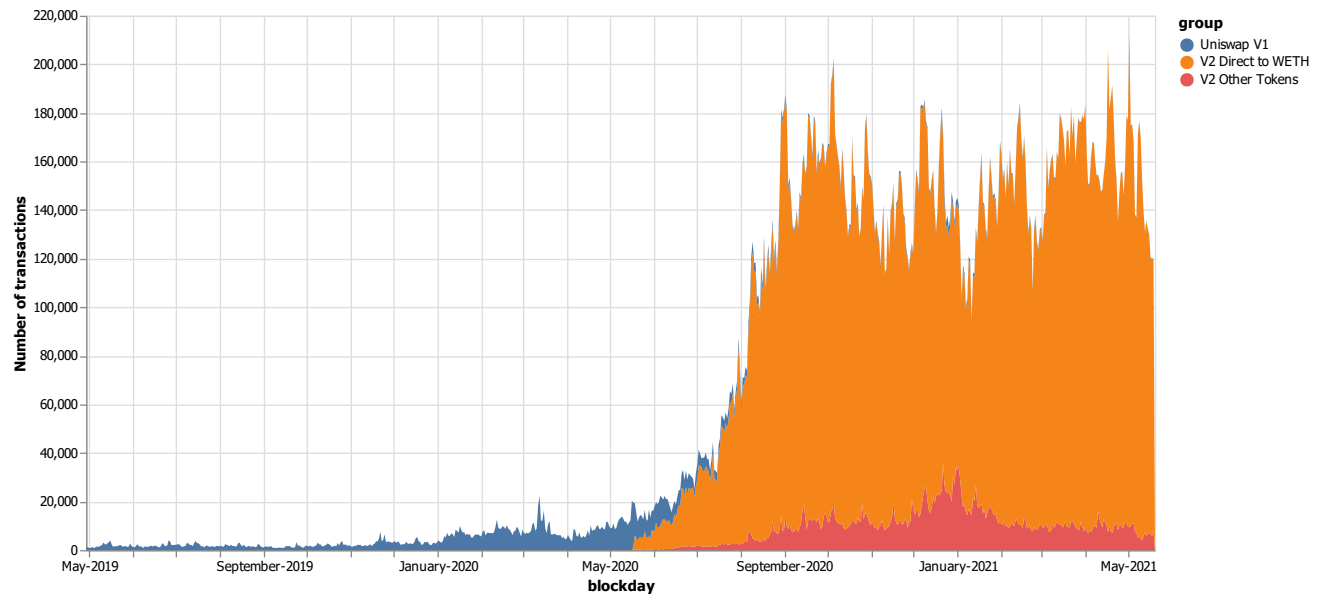
Figure 3. Number of transactions on Uniswap.
