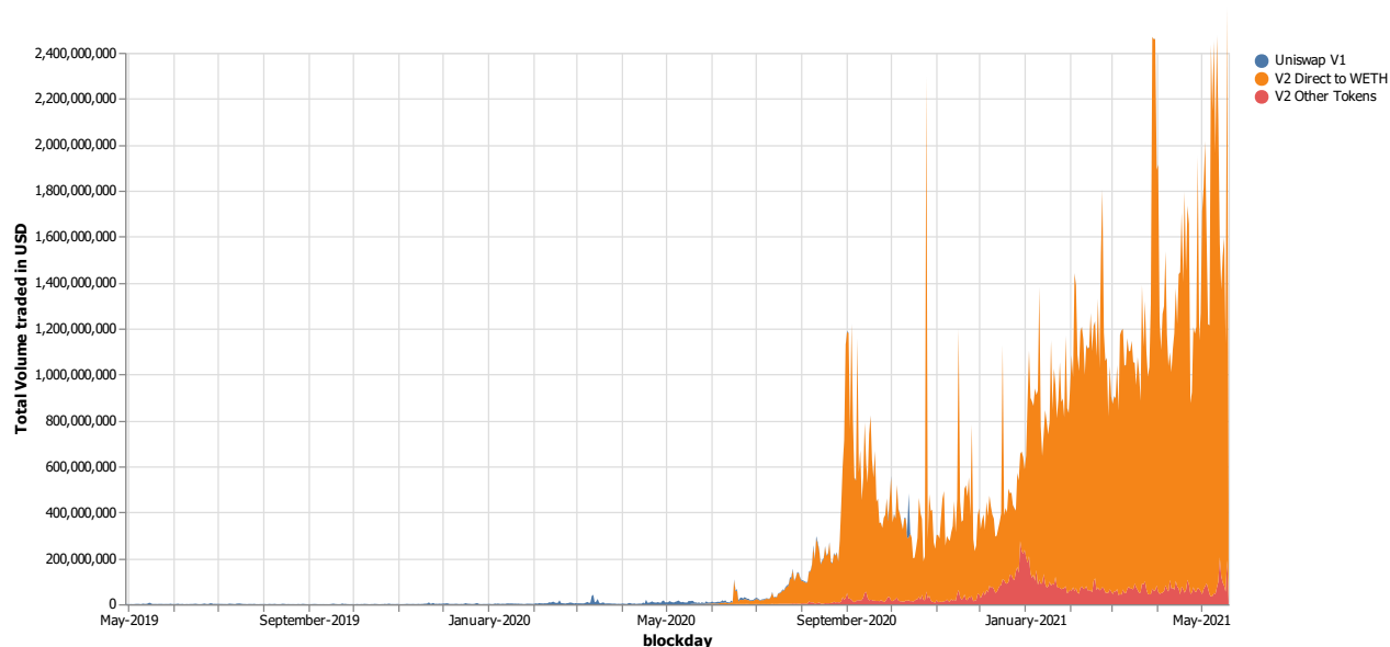
Figure 4. Trading volume on Uniswap The graph shows the daily volume of transactions including flash loans in USD capped at 2.4 billion USD.
