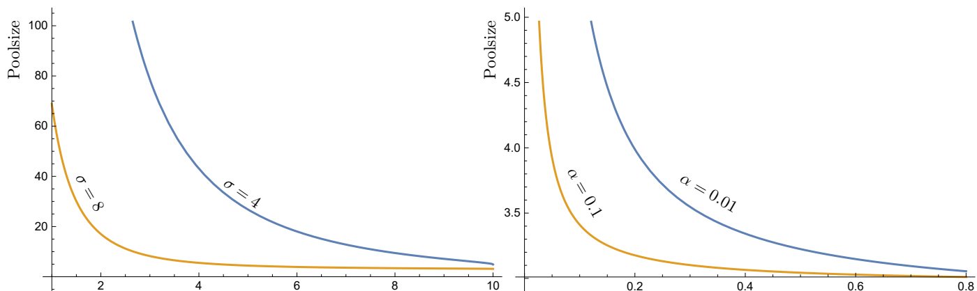
Figure 6. Poolsize as function of \sigma and \alpha . Unless otherwise stated the parameters are \alpha = 0.01 , P_0 = 10 , \sigma = 4 , q = 3 , \tau = 0.003
