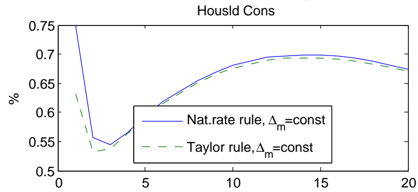
Figure 5: CREDIT MODEL – IRF to a technology shock
