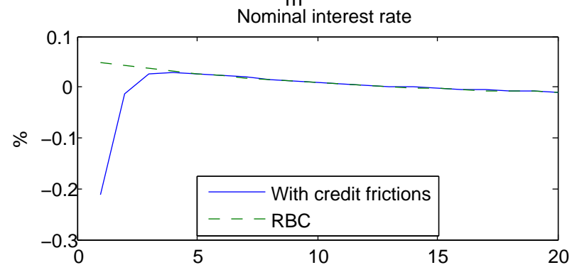
Figure 2: IRF to a technology shock – Nat.rate rule, \Delta_m = \text{const}
