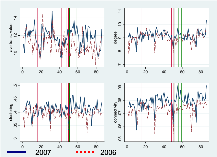
Figure 7: Development of a selection of traditional system measures and network properties over time: transaction value, degree, clustering, and connectivity.
