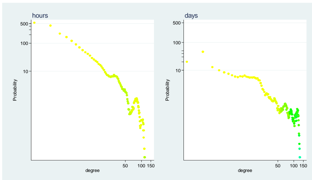
Figure 5: Degree distributions for time snapshots of one hour and one day, respectively
