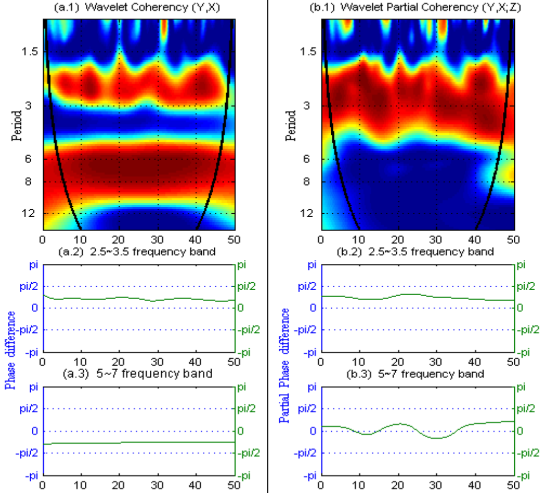
Figure 6: (a) Wavelet coherence between x_t and y_t ; (b) Wavelet partial coherence between x_t and y_t , after controlling for z_t ; (a.2) - (a.3) Phase-difference; (b.2) - (b.3) Partial phase-difference.
