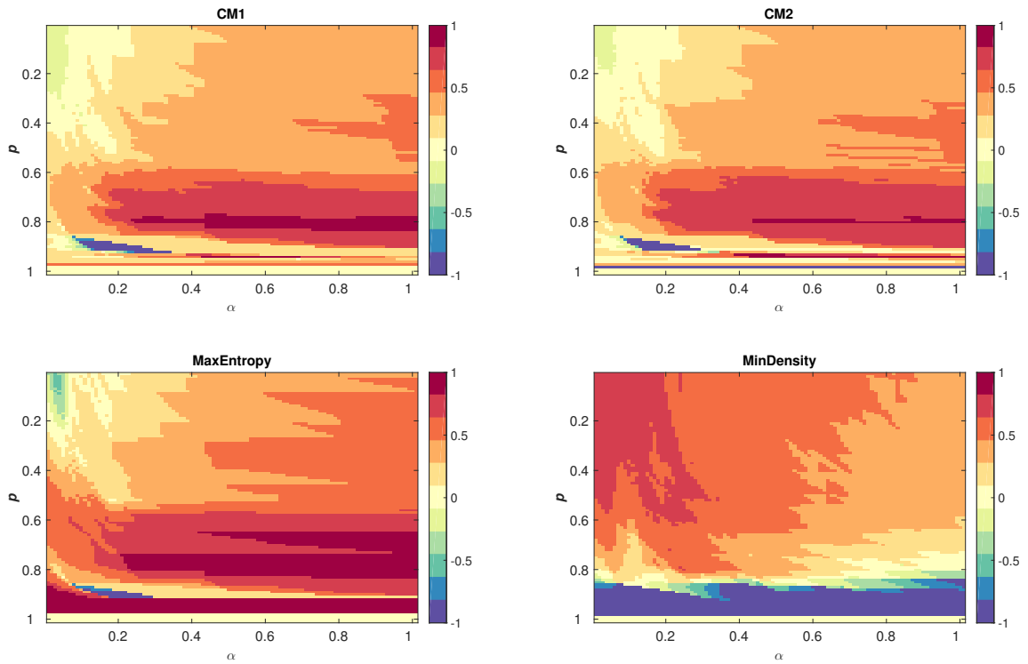
Figure 7: Relative difference of the probability of default between actual network and the null models ( D_r ) at the aggregated level for \alpha \in [0,1] (small to large market impact) and p \in [0,1] (large to small initial shock). Data for year 2010. Warm color corresponds to an underestimation of the actual network, while cold color indicates an overestimation.
