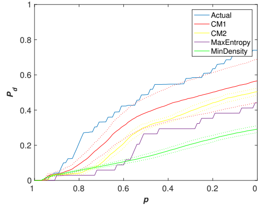
(b) \mathbf{W} , \alpha = 0.5
