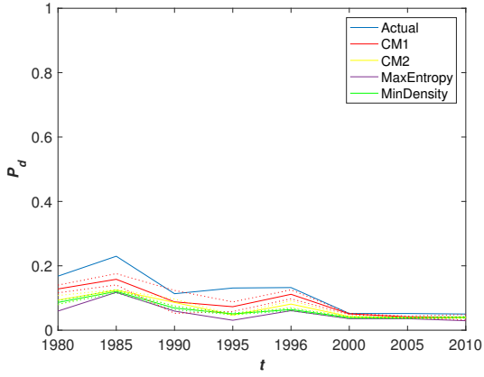
(a) \mathbf{W} , p = 0.8
