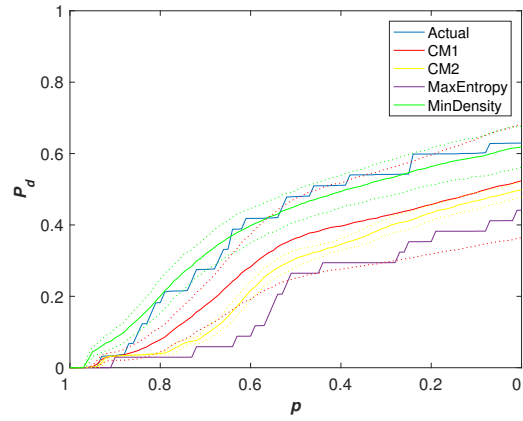
(f) \mathbf{W} \rightarrow \mathbf{W}^{\mathbf{I}} , \alpha = 0.5
