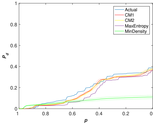
(c) \mathbf{W}^{\mathbf{I}} , \alpha = 0.1
