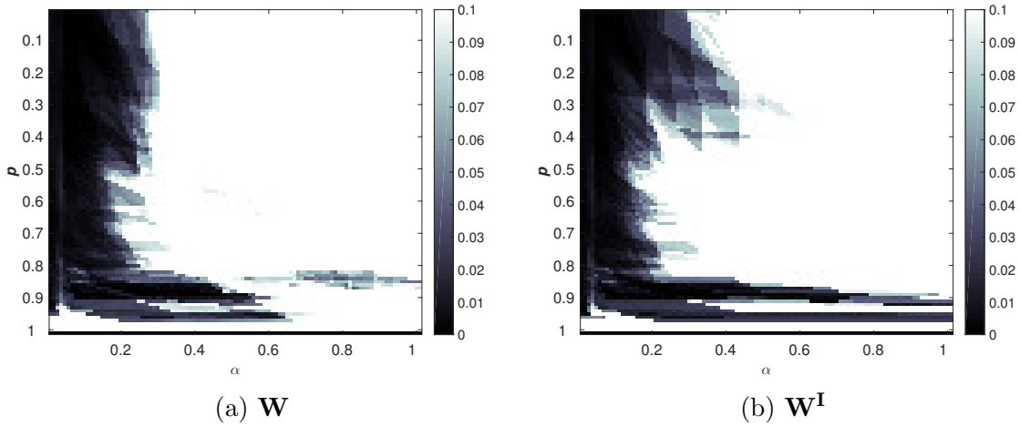
Figure 5: Trend analysis. p -value of regression analysis of P_d against a constant and a time variable (year), for different combinations of p and \alpha . Darker color denotes a smaller p -value.
