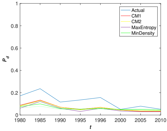
(c) \mathbf{W}^I , p = 0.8
