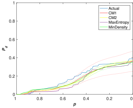
(e) \mathbf{W} \rightarrow \mathbf{W}^{\mathbf{I}} , \alpha = 0.1
