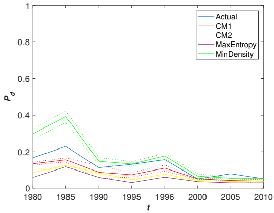
(e) \mathbf{W} \rightarrow \mathbf{W}^I , p = 0.8
