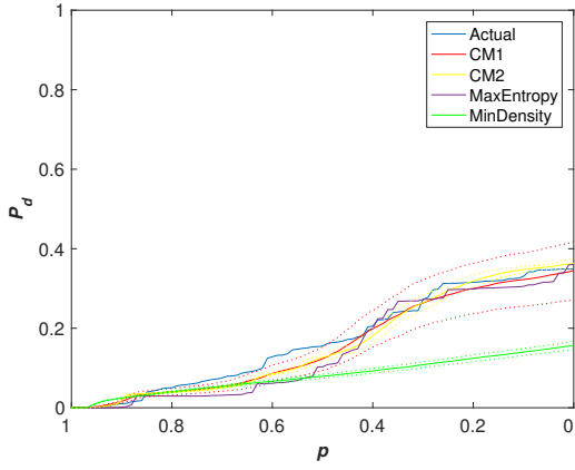
(a) \mathbf{W} , \alpha = 0.1
